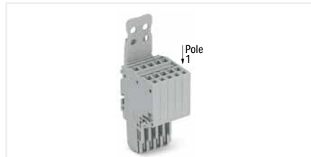
2-conductor female plugs; with locking levers and strain relief plates
