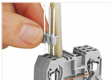
Inserting a pin module into 280 Series blocks.
