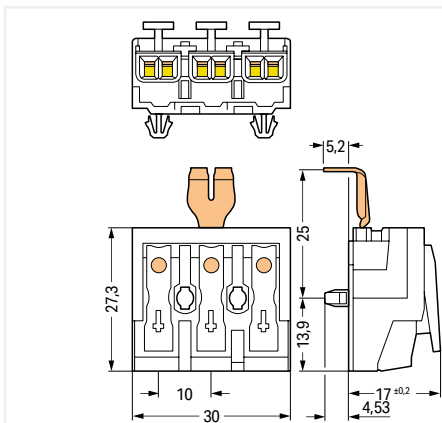
Field-wiring terminal block; with ground contact; with snap-in mounting feet; 3-pole; white
