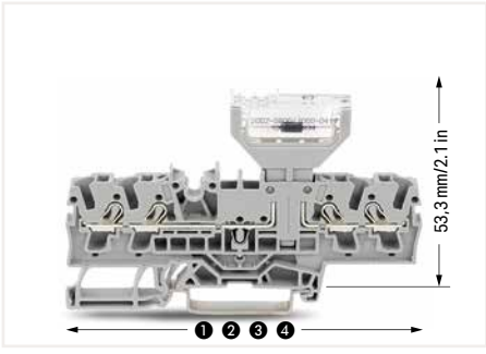
Lengths of carrier terminal blocks with a pluggable diode module:
