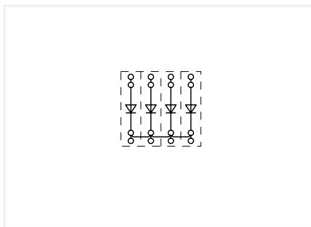
Polarized diode gates with a common cathode can be created using the following terminal blocks: 280-815/281-410 or 280-815/281-411
