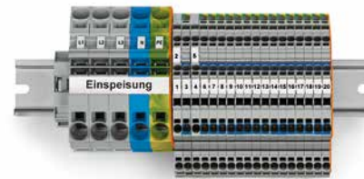
FI/LS main distribution board set TOPJOB® S
