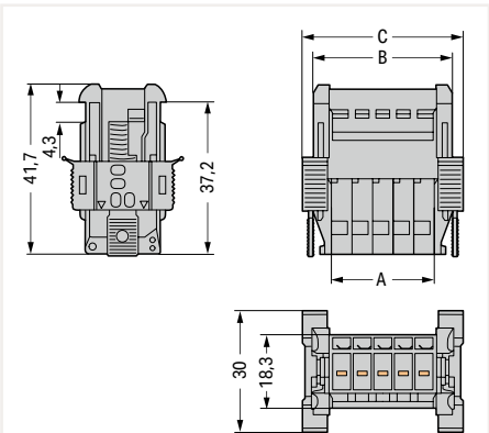
Insert a male connector with snap-in flanges (769-605/006-000) into the cutout.
