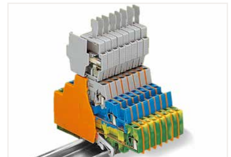
When triple-deck terminal blocks are used with a fuse plug (6 mm wide) in the receptacle (top) level, the extra width can be compensated for the 280 Series (5 mm wide) via an intermediate plate (1.1 mm thick).
