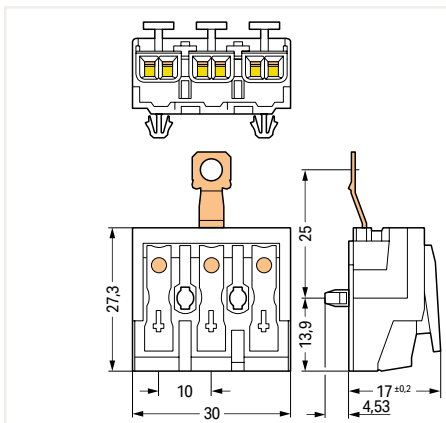
Field-wiring terminal block; with screw-type ground contact; with snap-in mounting feet; 3-pole; white
