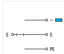
Actuator disconnect terminal block; with ground connection; for phase interruption
