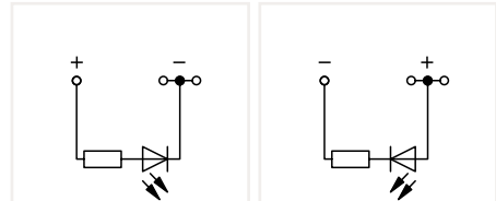
3-conductor LED terminal block; with red LED; gray
