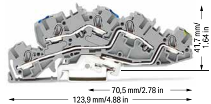
Multilevel installation terminal block; gray
