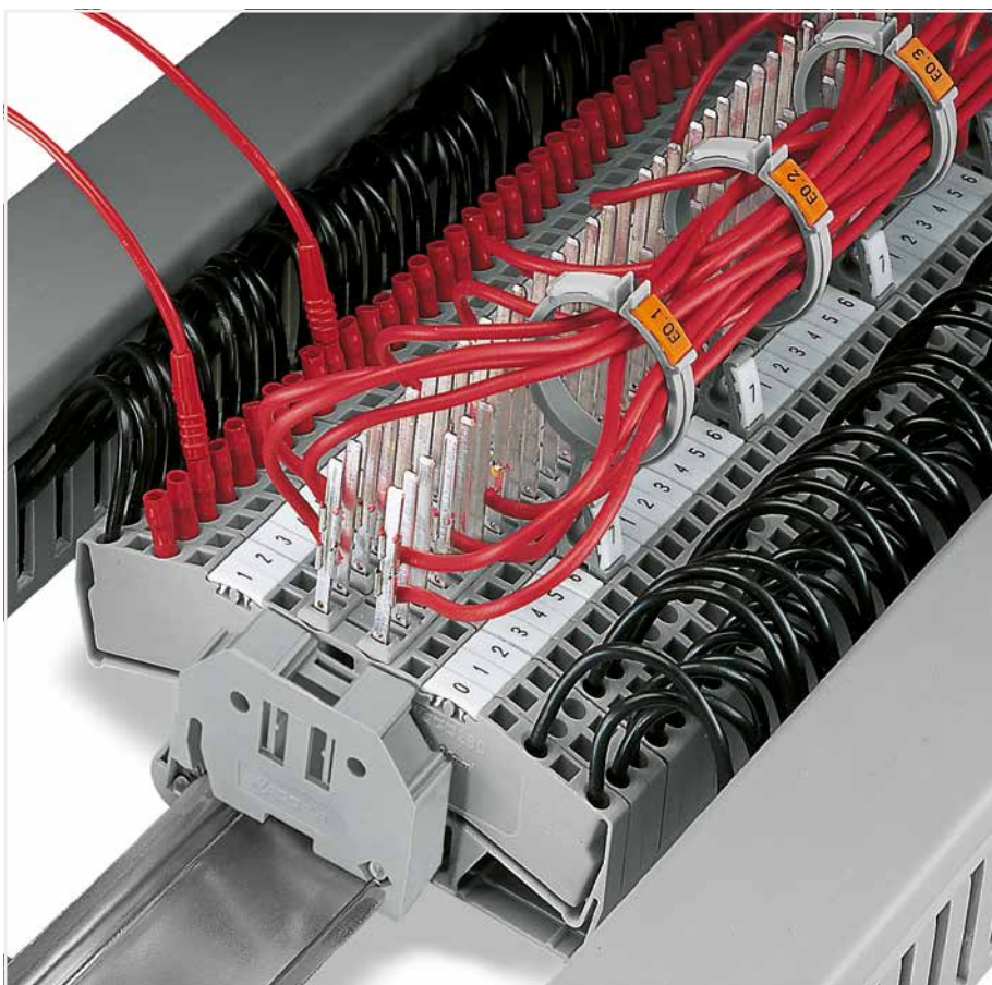
Terminal blocks for matrix patching: Inserting/removing a conductor in the terminal block's center.
