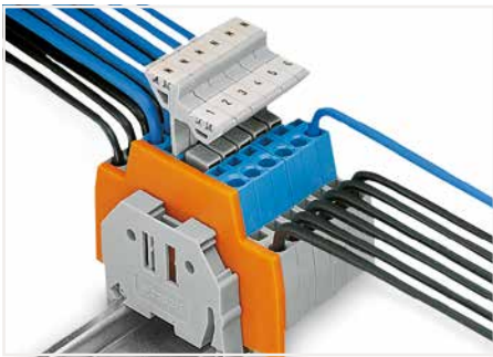
Double-deck terminal blocks used as control conductor terminal blocks (e.g., for magnetic valves) with the upper deck commoned.
