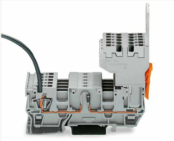
2-conductor female plug Diode carrier terminal blocks can be commoned via 280 and 780 Series Jumpers and tested using a test plug adapter (280-4..).
