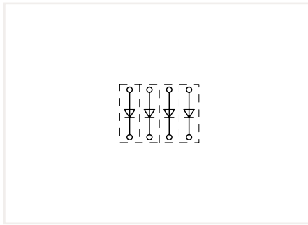
Open diode gates can be created using the following terminal blocks: 280-915/281-410 or 280-915/281-411
