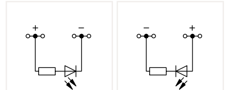
4-conductor LED terminal block; with red LED; gray
