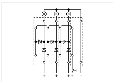
Lamp test circuits can be created using the following terminal blocks: 281-635/281-492 or 281-635/281-491
