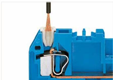
Insert stripped, untwisted conductor into insulation stop.
