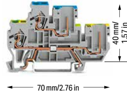
1-conductor/1-pin double-deck carrier terminal block; ground conductor/through terminal block; gray
