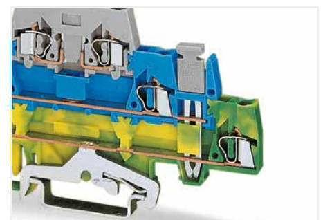
Grounding to DIN-rail: Connecting N-level to ground level via vertical jumper.
