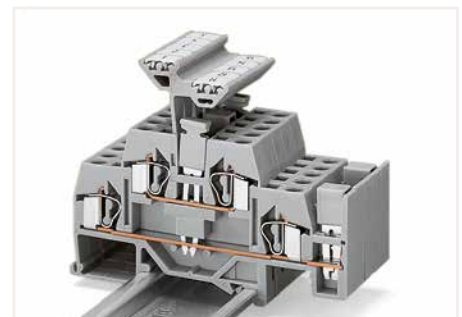
A vertical jumper allows commoning of upper and lower level, giving a 4-conductor commoned through terminal block in one housing. Two adjacent terminals may be commoned together on the same level using a push-in adjacent jumper.
