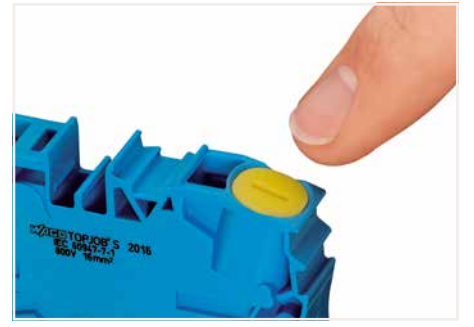
Finger guard seals an unused conductor entry.
