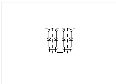
Polarized diode gates with a common cathode can be created using the following terminal blocks: 280-673/281-410 or 280-673/281-411
