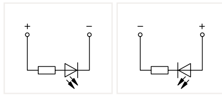
1-conductor/1-pin LED carrier terminal block; with two jumper positions
