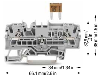
2-conductor fuse terminal block; for mini-automotive blade-style fuse; with test point Electrical ratings are given by the fuse. Blade-style fuses: Observe touch-proof protection for 42 V and higher voltages!
