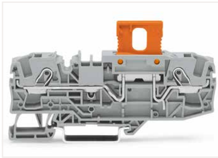
Carrier terminal block (2006-1661) with disconnect plug (2006-401) in operating position
