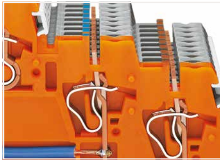
Commoning a supply voltage using unshielded push-in type jumper bars, 2- to 9-way or 17-way (2 x 8 bits), depending on application.
