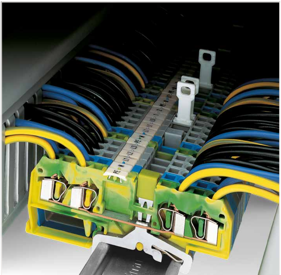
Steel DIN-rails are not suited for PEN (ground and N-conductor) applications per EN 60947-7-2 (VDE 0611, Part 3).
