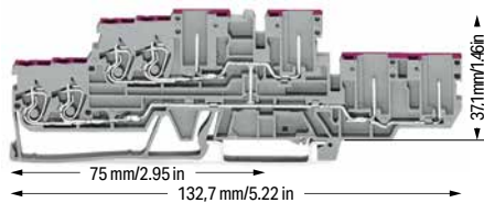
4-conductor/4-pin double-deck carrier terminal block; 4-conductor/4-pin through terminal block; internally commoned; Violet conductor entry; gray
