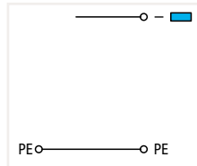
Actuator supply terminal block; with ground connection; power supply from control panel side; with end plate
