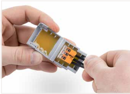
Place the wired connector in the Yellowox.
