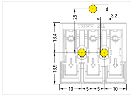
3-pole – with snap-in ground contact, d = 4.9 mm with screw-type ground contact, d \leq 4.1 mm
