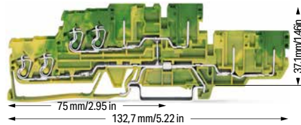
4-conductor/4-pin double-deck carrier block; 4-conductor/4-pin ground conductor block; internally commoned; green-yellow
