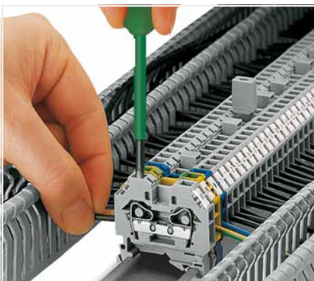
CAGE CLAMP® connection Inserting a conductor. With ferruled conductors, it is necessary to use a terminal block one size larger than the conductor's nominal cross section.
