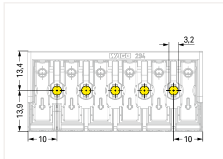
6-pole – without ground contact
