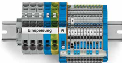
Subdistribution board set TOPJOB® S
