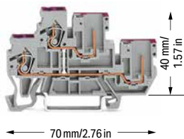
2-conductor/2-pin double-deck carrier terminal block; 2-conductor/2-pin through terminal block; internally commoned; Violet conductor entry; gray
