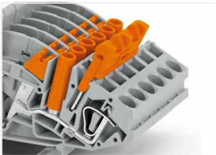
Jumper with safety lid Jumper in pre-locked position
