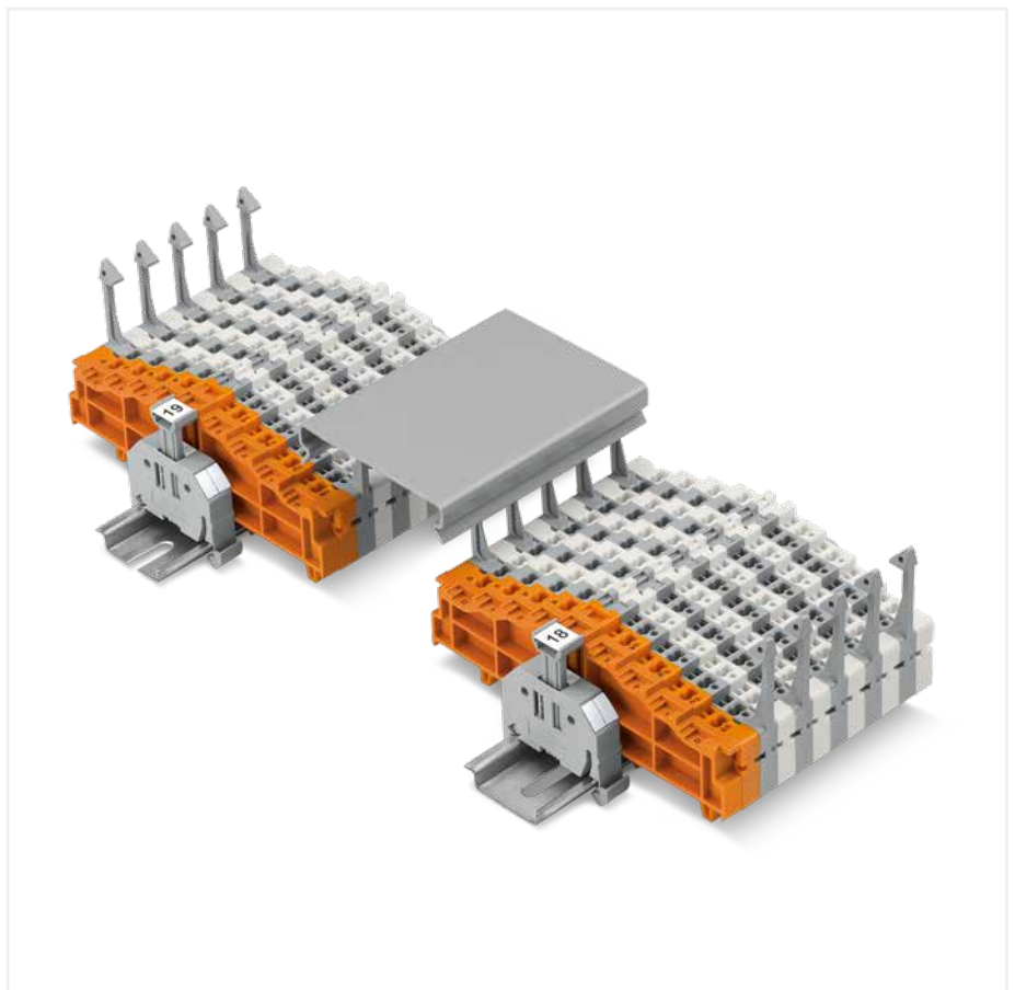
Open the assembly by laterally sliding a block via operating tool (2.5 x 0.4 mm blade).
