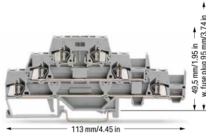
Triple-deck terminal block; through/through/carrier terminal block for fuse plugs; with slot for adjacent jumper on lower level
