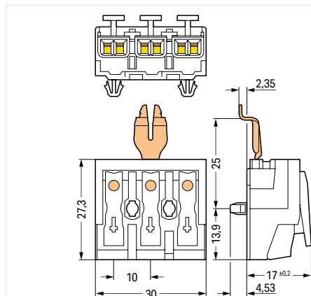
Field-wiring terminal block; with angled ground contact; with snap-in mounting feet; 3-pole; white
