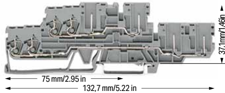
2-conductor/2-pin double-deck carrier terminal block; through/through terminal block; gray
