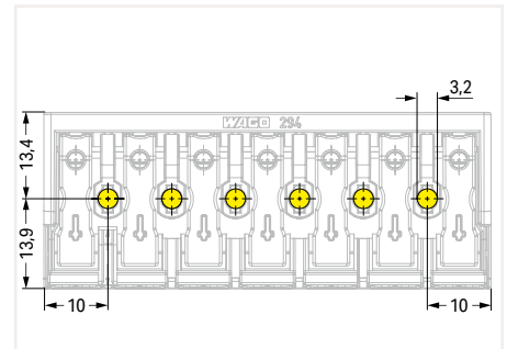
7-pole – without ground contact
