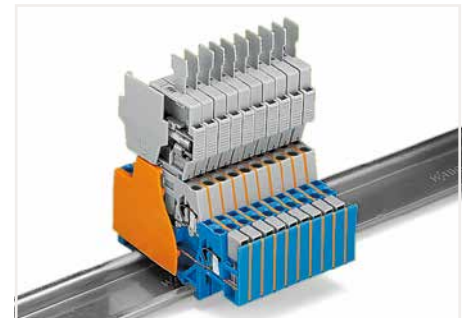
When double-deck terminal blocks are used with a fuse plug (6 mm wide) in the receptacle (top) level, the extra width can be compensated for the 280 Series (5 mm wide) via an intermediate plate (1.1 mm thick). If required, this special intermediate plate still allows commoning on the lower level via push-in adjacent jumpers (280-402).
