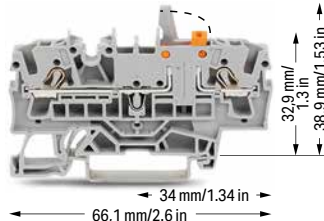
2-conductor disconnect/test terminal block; with mechanical interlock; with test point; orange disconnect link
