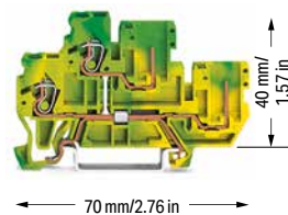
2-conductor/2-pin double-deck carrier block; 2-conductor/2-pin ground conductor block; internally commoned; green-yellow
