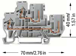
1-conductor/1-pin double-deck carrier terminal block; through/through terminal block; gray
