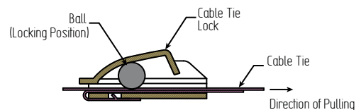
2) Locking Position
